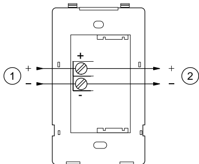
Figure 3: Wiring diagram
