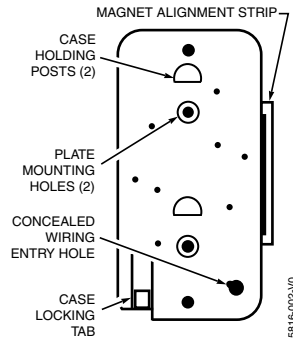
Figure 1. Mounting Plate
