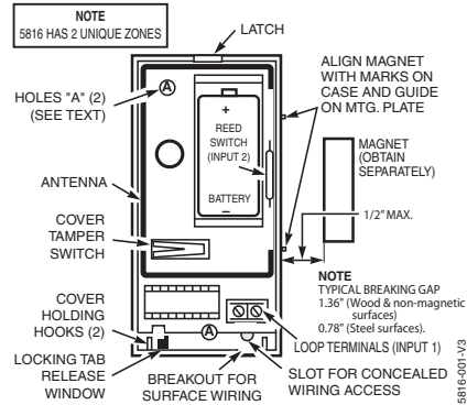
Figure 2. Transmitter, Cover Removed
