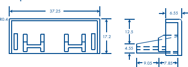
Tapa final
