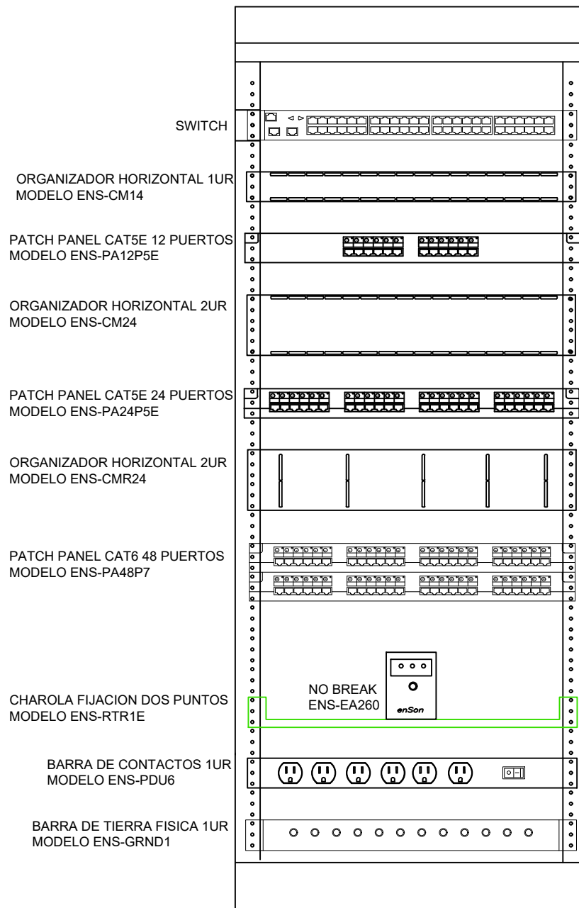
ENS-RACK248
